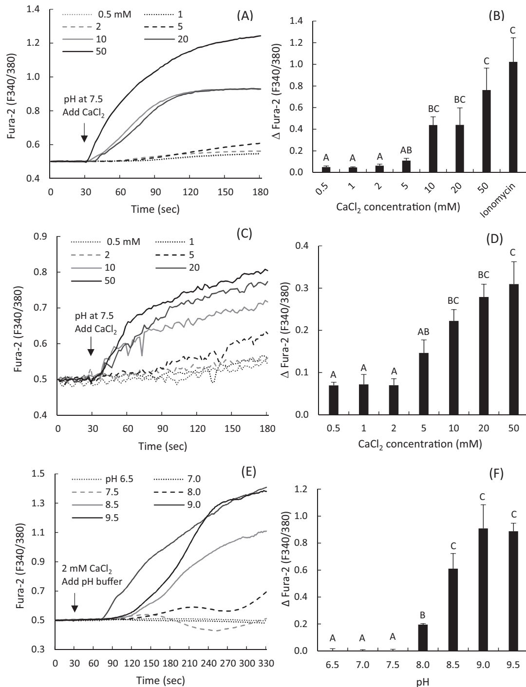
Figure 3. Increases in intracellular \text{Ca}^{2+} concentration of sperm from Redtail Splitfin. (A) Average \text{Ca}^{2+} signals of sperm within bundles during stimulation with different \text{CaCl}_2 concentrations at pH 7.5. (B) Average peak increases of sperm within bundles for each \text{CaCl}_2 concentration compared with 1 \mu\text{M} ionomycin. (C) Average \text{Ca}^{2+} signals of dissociated single sperm cell from bundles during stimulation with different \text{CaCl}_2 concentrations at pH 7.5. (D) Average peak increases of dissociated single sperm cells from bundles for each \text{CaCl}_2 concentration. (E) Average \text{Ca}^{2+} signals of sperm within bundles during stimulation (0–330 s) with different pH in the presence of 2 \text{ mM} \text{CaCl}_2 . (F) Average peak increases of sperm within bundles for each pH level. Bars represent means \pm SEM; n = 50 – 150 regions of interest per male from three males. Values sharing letters were not significantly different.
