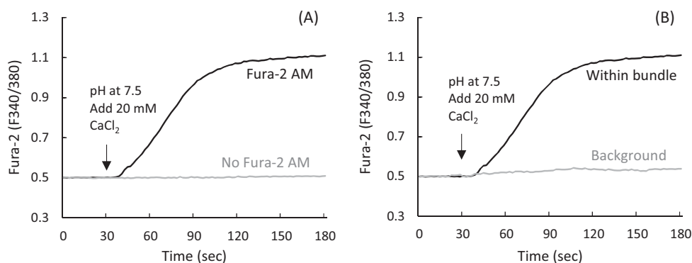
Figure 4. Effect of autofluorescence and background on \text{Ca}^{2+} signals. (A) Increase in intracellular \text{Ca}^{2+} by 20 mM \text{CaCl}_2 (pH = 7.5) in bundles with Fura-2 AM loading (black line) and without (gray line, autofluorescence). (B) Increase in intracellular \text{Ca}^{2+} by 20 mM of \text{CaCl}_2 (pH = 7.5) in bundles (black line) and from background areas outside of bundles (gray line).
