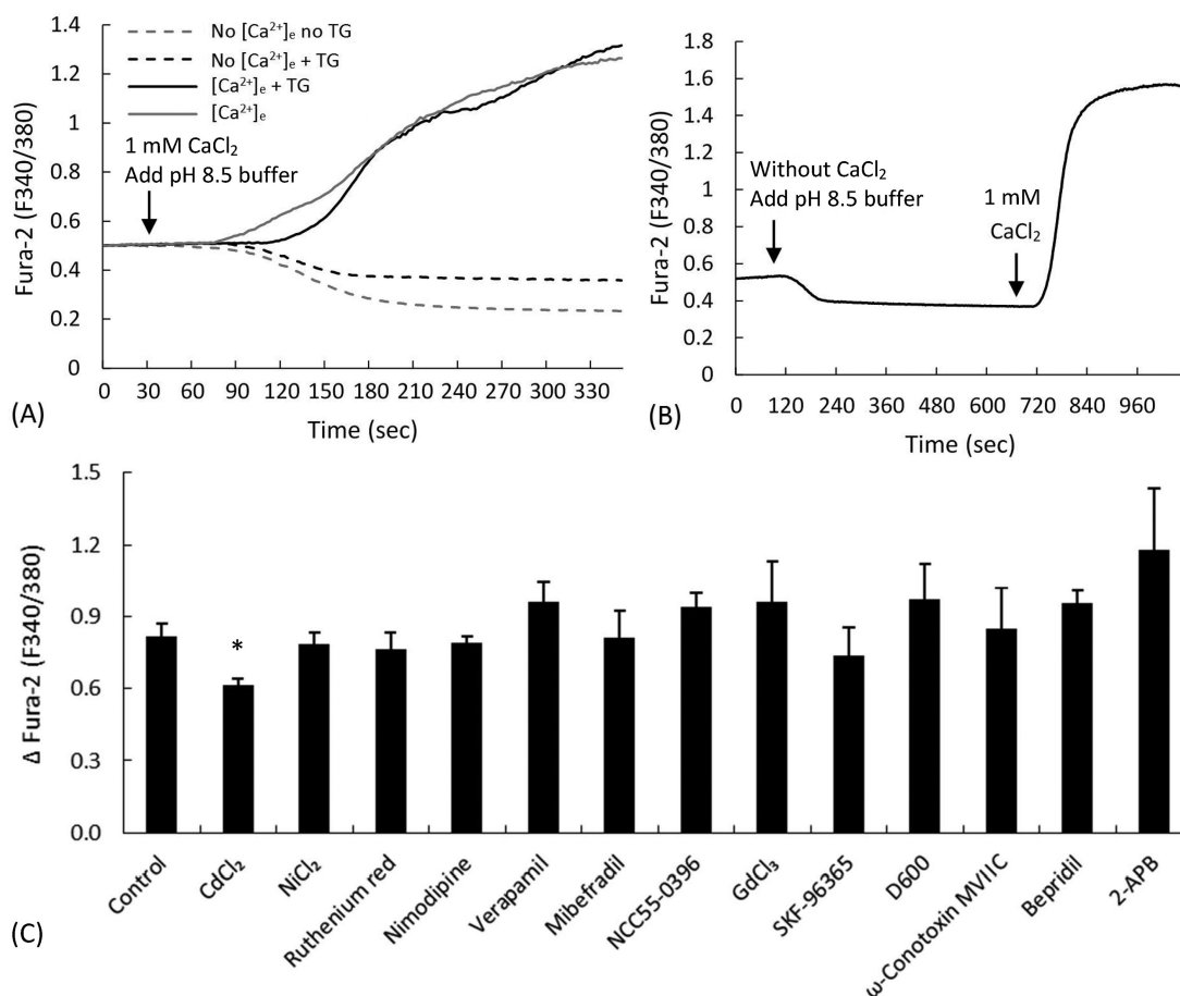
Figure 5. Intracellular \text{Ca}^{2+} increase is dependent on extracellular sources and the increases were not inhibited by major \text{Ca}^{2+} channel blockers. (A) Thapsigargin (TG, 1 \mu\text{M} ) was added to bundle suspensions with or without 1 mM \text{CaCl}_2 to deplete intracellular \text{Ca}^{2+} stores prior increase of pH to 8.5. (B) Addition of 1 mM \text{CaCl}_2 to the extracellular buffer increased \text{Ca}^{2+} influx after stimulation with pH 8.5 under \text{Ca}^{2+} -free conditions. (C) Bundles were pretreated the respective blockers ( \text{CdCl}_2 (200 \mu\text{M} ), \text{NiCl}_2 (300 \mu\text{M} ), ruthenium red (10 \mu\text{M} ), nimodipine (30 \mu\text{M} ), verapamil (30 \mu\text{M} ), mibefradil (40 \mu\text{M} ), NNC 55-0396 (10 \mu\text{M} ), \text{GdCl}_3 (100 \mu\text{M} ), SKF-96365 (100 \mu\text{M} ), methoxyverapamil (D600 30 \mu\text{M} ), \omega -Conotoxin MV1IC (2 \mu\text{M} ), bepridil (50 \mu\text{M} ), or 2-APB (300 \mu\text{M} ) for 20 min prior to stimulation by extracellular exposure to 1 mM \text{CaCl}_2 stimulation and pH 8.5. Bars represent means \pm SEM; n = 50 –150 regions of interest per male from three males. Only \text{CdCl}_2 treatment (asterisk) produced a significant reduction in relation to the control group (without blocker) and blockers.
